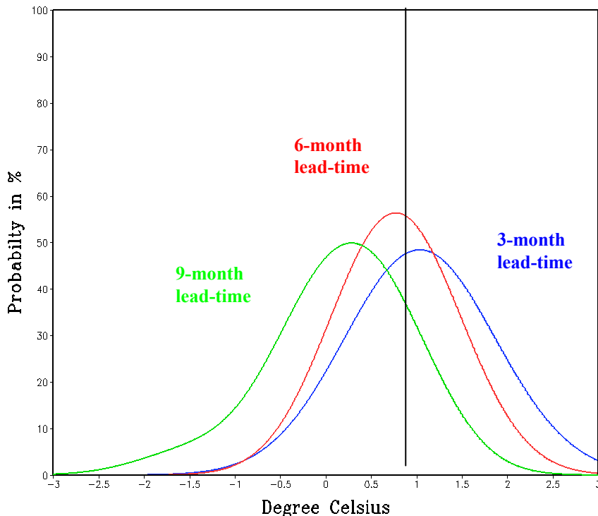
FIGURE 2.8 Examples of probabilistic predictions for Nino3.4 SST anomaly, represented by probability density functions (PDFs). The green curve is the prediction with the longest lead time (9 months), followed by the red (6 months) and blue (3 months) curves. With shorter lead times, the PDF for the prediction shifts to progressively warmer temperatures. The observed value for Nino3.4 SST anomaly is indicated by the vertical black line (0.78°C). SOURCE: International Research Institute for Climate and Society (IRI).
