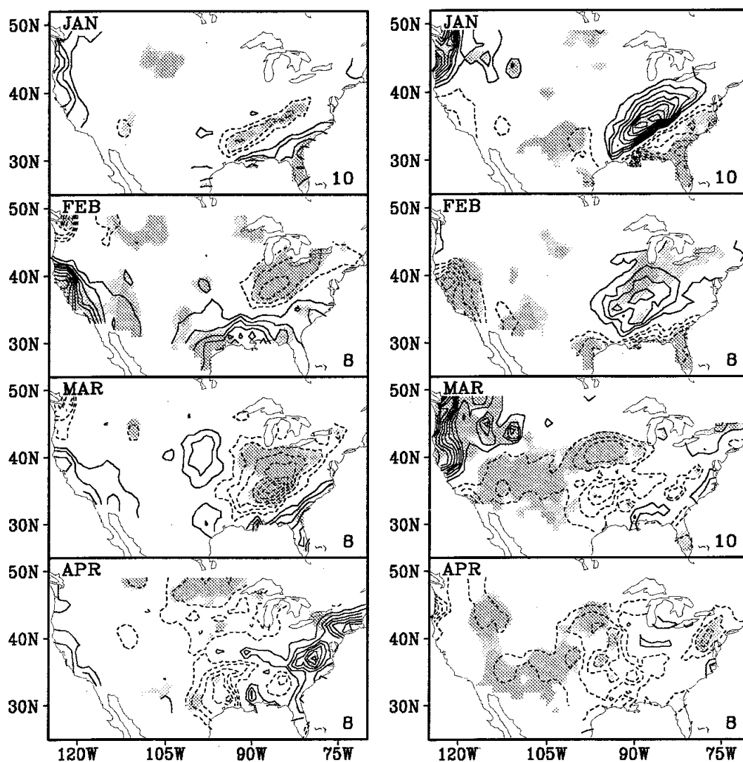
FIGURE 3.7. Composites of monthly-mean precipitation anomalies associated with months experiencing warm SST (left column) or cold SST (right column) in the tropical Pacific for January through April. These maps illustrate that opposite signed SST anomalies do not necessarily produce opposite signed precipitation anomalies (e.g., the areas experiencing wetter-than-average conditions when SST is warm are not necessarily drier-than-average when SST is cold, and vice versa). Contour interval is 10 mm of precipitation; solid contours are for wet anomalies; dashed contours are for dry anomalies. Shading indicates areas of statistical significance. SOURCE: Adapted from Livezey et al. (1997).
