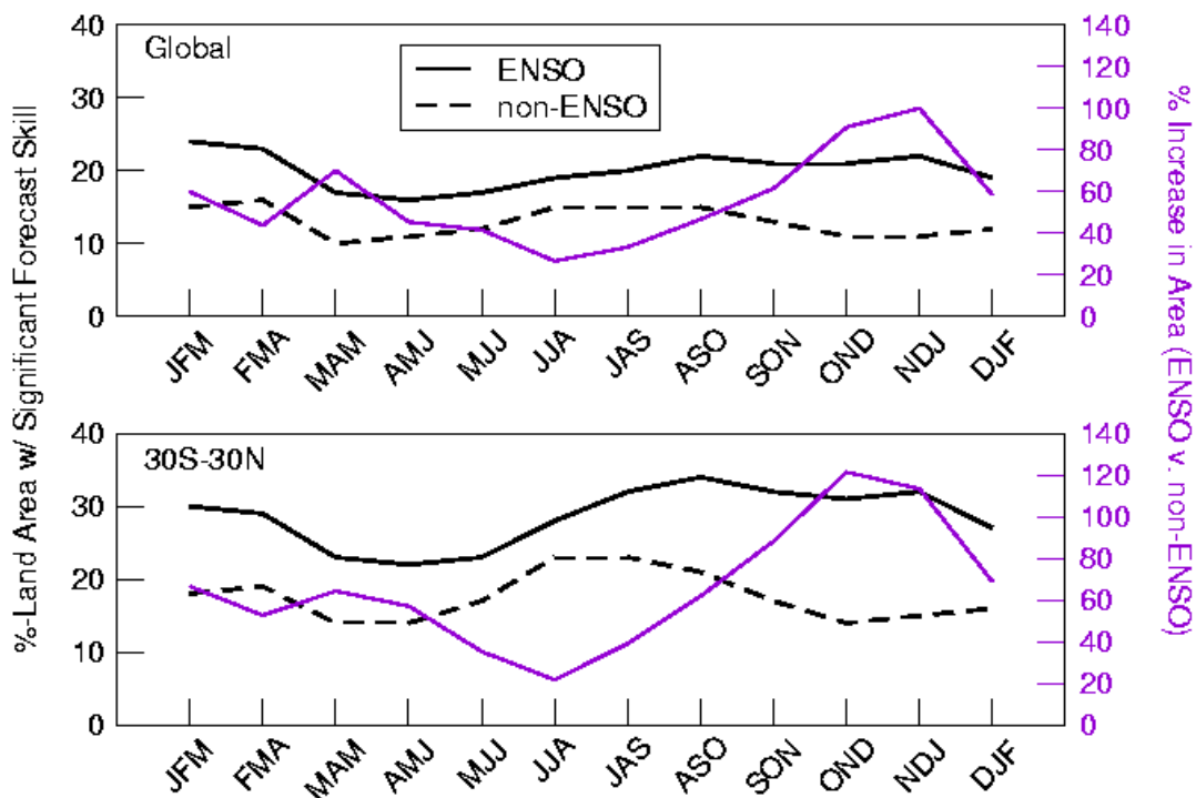
FIGURE 3.13 Seasonal precipitation forecasts are skillful over a larger portion of land during ENSO events (solid black line) than ENSO-neutral conditions (dashed black line). The purple line indicates the percentage increase in area between ENSO events and ENSO-neutral conditions. Top panel corresponds to the entire globe; bottom panel the area within 30° latitude of the equator. SOURCE: Goddard and Dilley (2005).
