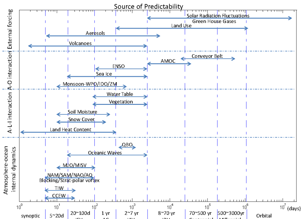
FIGURE 2.4 Processes that act as sources of ISI climate predictability extend over a wide range of timescales, and involve interactions among the atmosphere, ocean, and land. CCEW: convectively coupled equatorial waves (in the atmosphere); TIW: tropical instability wave (in the ocean); MJO/MISV: Madden-Julian Oscillation/Monsoon intraseasonal variability; NAM: Northern Hemisphere annular mode; SAM: Southern Hemisphere annular mode; AO: Arctic oscillation; NAO: North Atlantic oscillation; QBO: quasi-biennial oscillation, IOD/ZM: Indian Ocean dipole/zonal mode; AMOC: Atlantic meridional overturning circulation. For the y-axis, “A” indicates “atmosphere;” “L” indicates “land;” “I” indicates “ice;” and, “O” indicates “ocean.”
