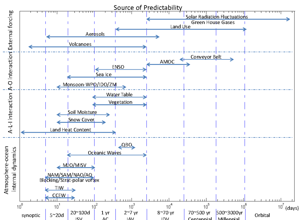
FIGURE S.1 Processes that act as sources of ISI climate predictability extend over a wide range of timescales and involve interactions among the atmosphere, ocean, and land. CCEW: convectively coupled equatorial waves; TIW: tropical instability wave; MJO/MISV: Madden-Julian Oscillation/Monsoon intraseasonal variability; NAM: Northern Hemisphere annular mode; SAM: Southern Hemisphere annular mode; AO: Arctic oscillation; NAO: North Atlantic oscillation; QBO: quasi-biennial oscillation, IOD/ZM: Indian Ocean dipole/zonal mode; AMOC: Atlantic meridional overturning circulation. For the y -axis, “A” indicates “atmosphere,” “L” indicates “land,” “I” indicates “ice,” and, “O” indicates “ocean.”
