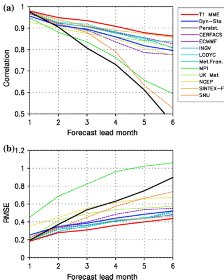
FIGURE 2.9 An example of a multi-model ensemble (MME) outperforming individual models in forecasting. (a) Anomaly correlation; the red line (MME) is above the individual models (colored lines), demonstrating that the pattern of anomalous temperature from the ensemble is a closer match to observations. (b) RMSE of NINO3.4; the red line is below the individual models, demonstrating that the magnitude of the errors associated with the ensemble is smaller. Black represents a persistence forecast. Names of the individual coupled models shown in the legend. SOURCE: Figure 7, Jin et al. (2008)
